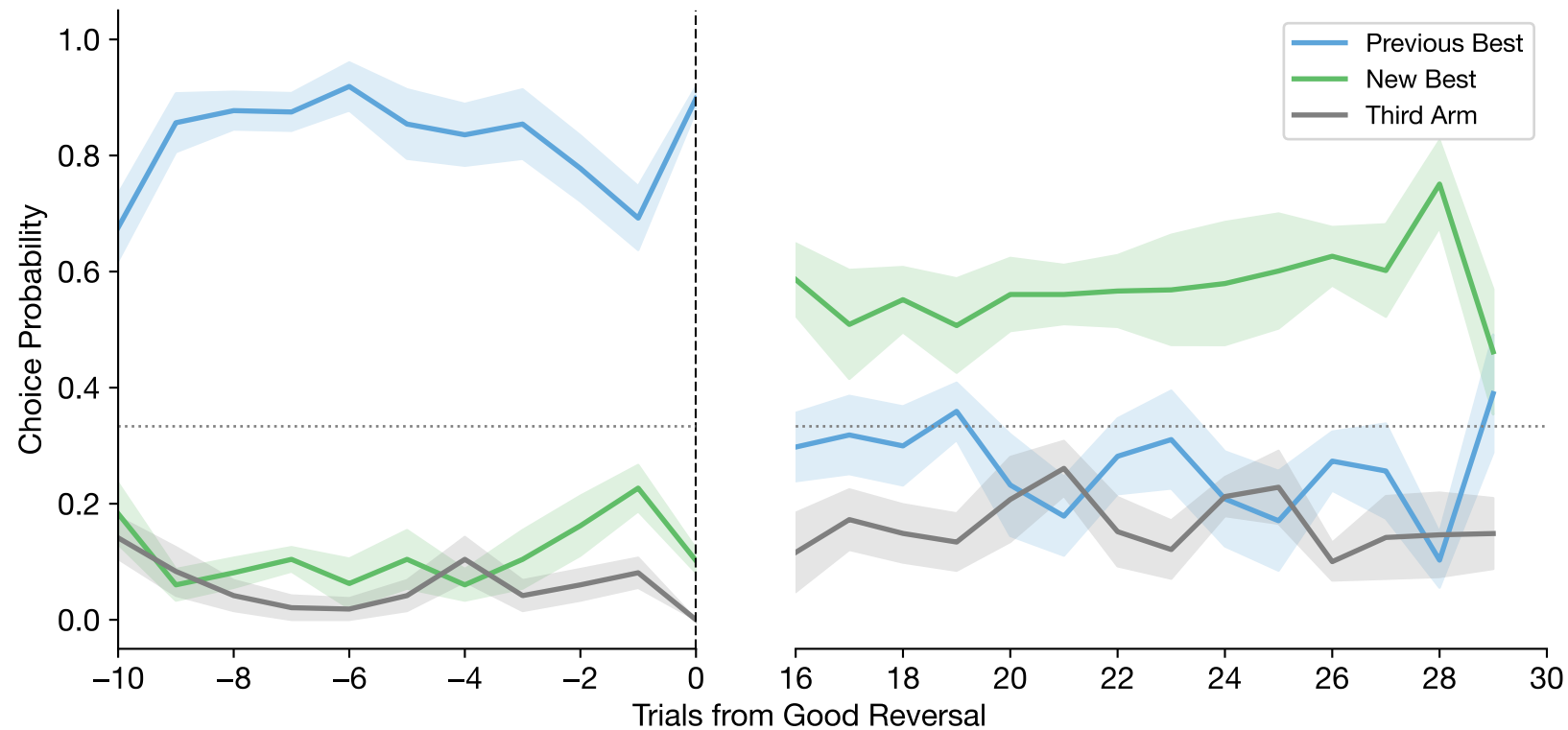
Good Reversal-Aligned Choices (mean \pm se across subjects | n=6 subjects, n=49 reversals) (Skipping first 15 trials post-reversal)
